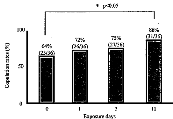
Fig. 3. Cumulative effect of electric field exposure of C57BL/6J males on the copulation rate with superovulated females.
