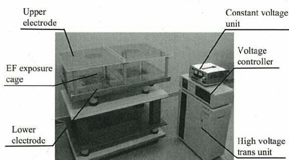
Fig. 1. The electric field exposure system. The electric field exposure system consists of electric exposure cages (also see Fig. 2), a constant voltage unit, high voltage transformer unit and voltage controller.
