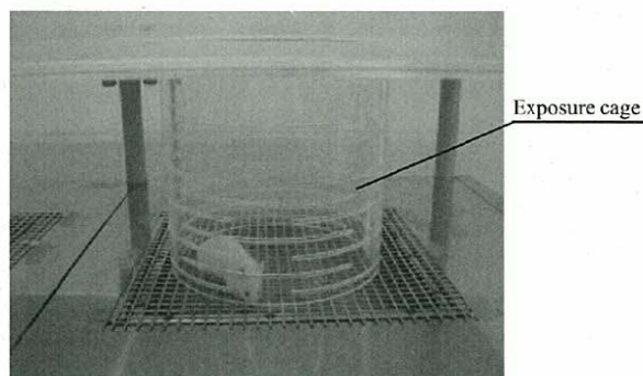
Fig. 2. The electric field exposure cage. A cylindrical plastic cage is placed between upper and lower stainless steel electrodes. The cylindrical cage has slits (length: 100 mm; width: 5 mm) at approximate intervals of 5 mm from each other to prevent smudges, due to feces and saliva, which might disturb the formation of a stable electric field.
