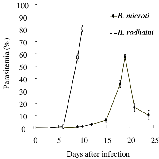
Fig.1. Changes of parasitemia in B. microti and B. rodhaini infected mice.
