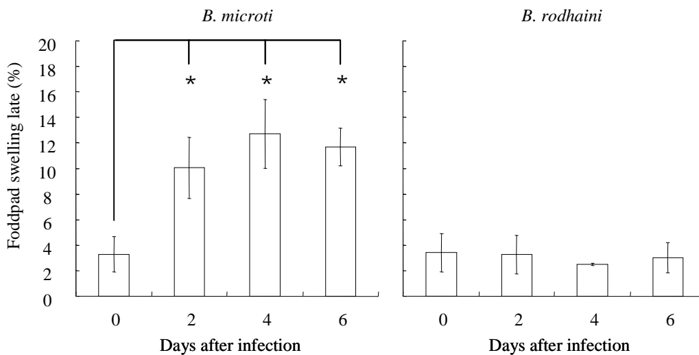
Fig.2. Delayed-type hypersensitivity responses in B. microti and B. rodhaini infected mice. * : Significant increase ( p < 0.05 ) compared to the initial level.
