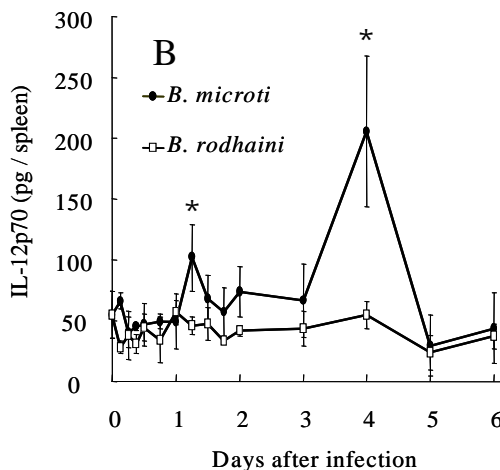
Fig.5 Changes of Serum (A) and splenic (B) IL-12p70 concentrations in B. microti - and B. rodhaini - infected BALB/ mice.
