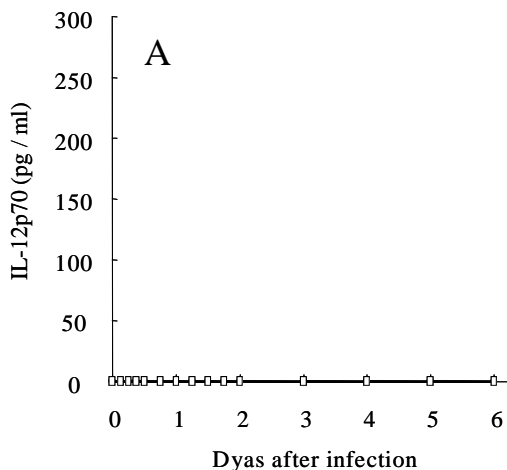
Fig.5 Changes of Serum (A) and splenic (B) IL-12p70 concentrations in B. microti - and B. rodhaini - infected BALB/ mice.
