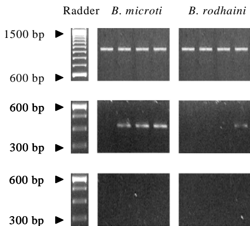
Fig.3. Expressions of IFN- \gamma mRNA and IL-4 mRNA in splenic CD4 positive T cells from mice infected with B. microti and B. rodhaini .
